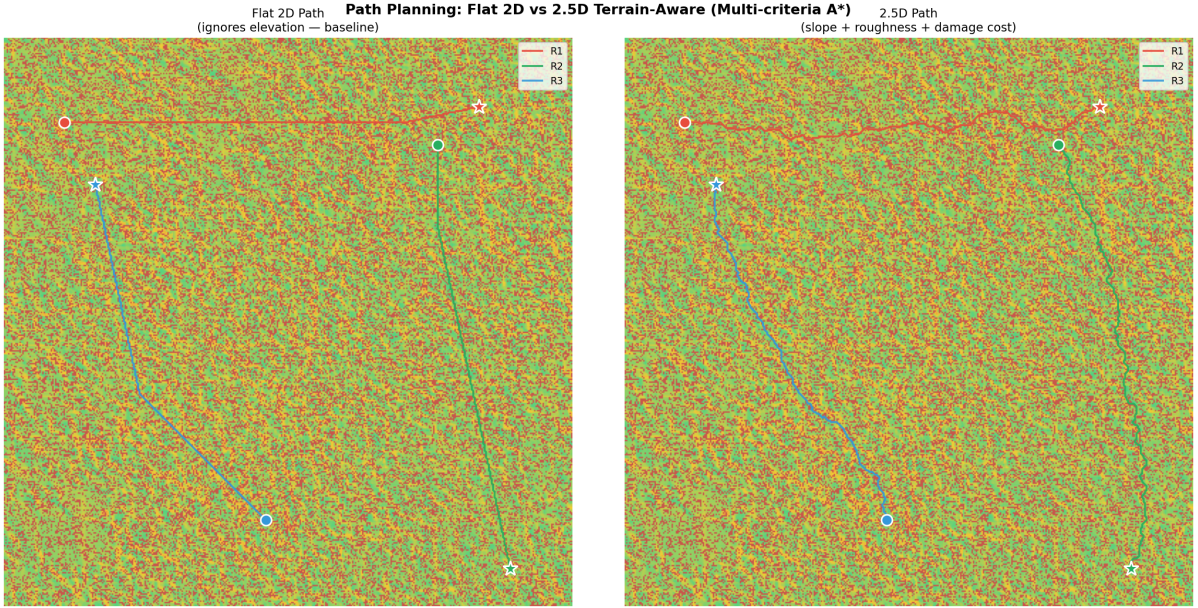
Figure 1: Illustrative output: 2D vs 2.5D path planning. The 2.5D-aware planner avoids steep slopes and rough areas, even if the Euclidean distance is longer.
